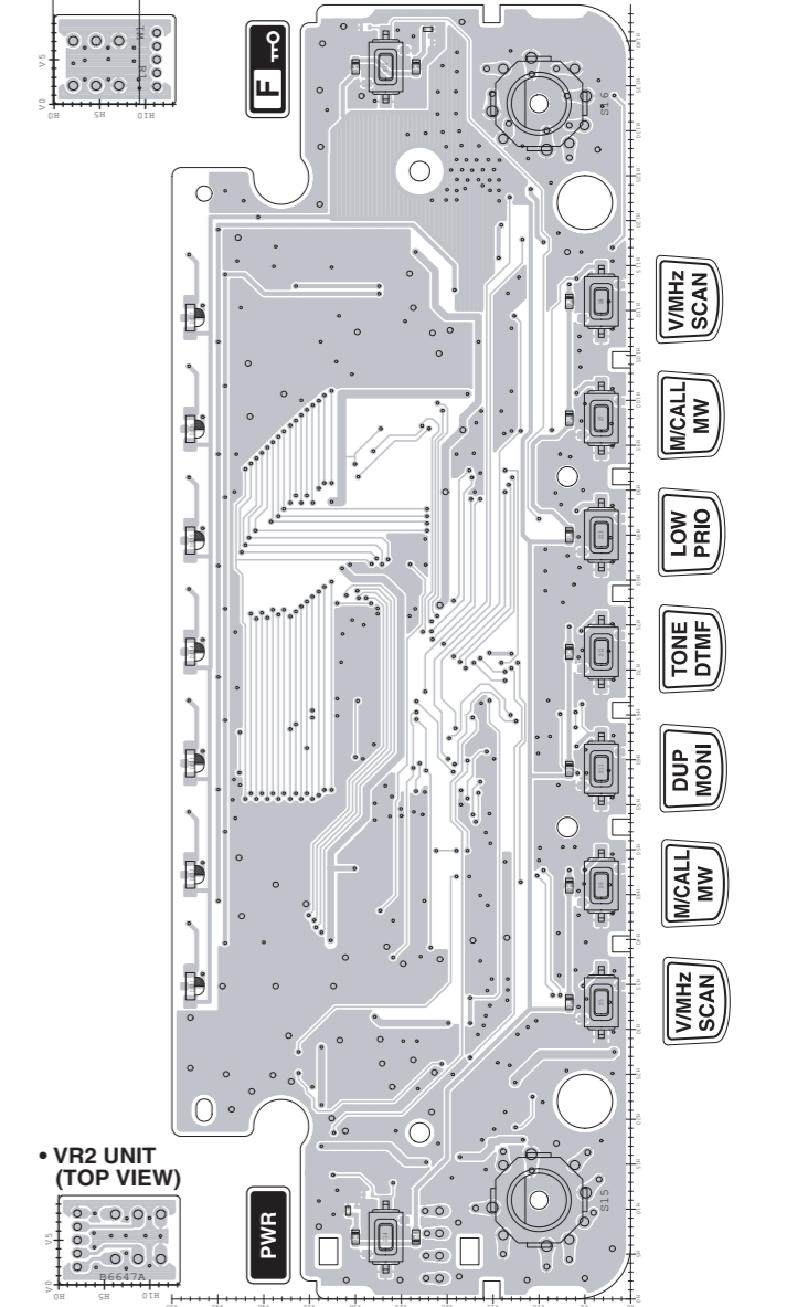
• CONTROL UNIT (TOP VIEW)
